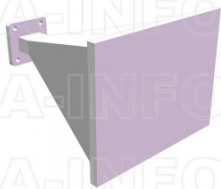
LB-75-20-ASPO Standard Gain Horn Antenna 10-15GHz 20dB Gain Rectangular Waveguide Interface
